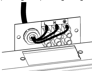
Figure 5: Electrical Connection
