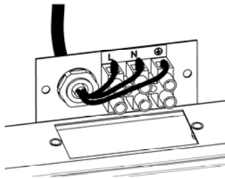
Figure 5: Electrical Connection
